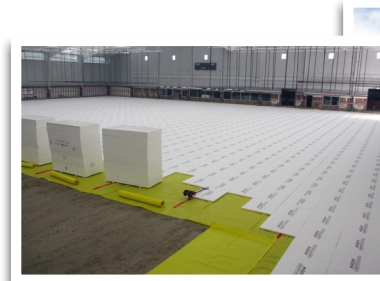
Perimeter/Under-slab
